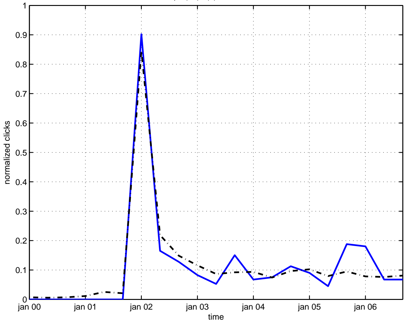
spin(32)/z(2) fibre bundle
