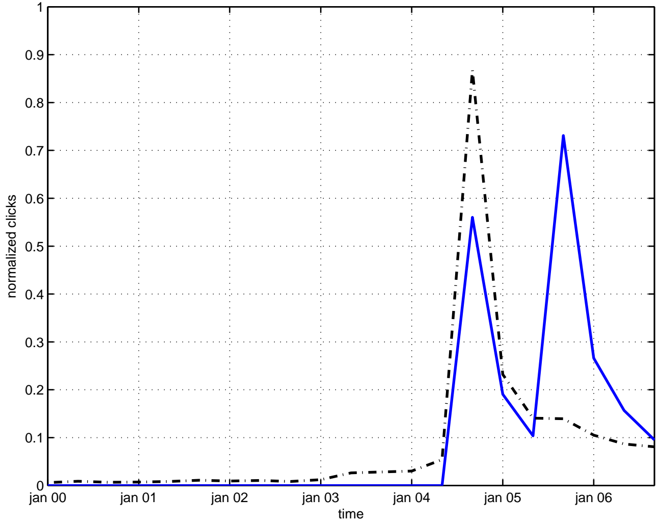
spin(10) gauge field theory
