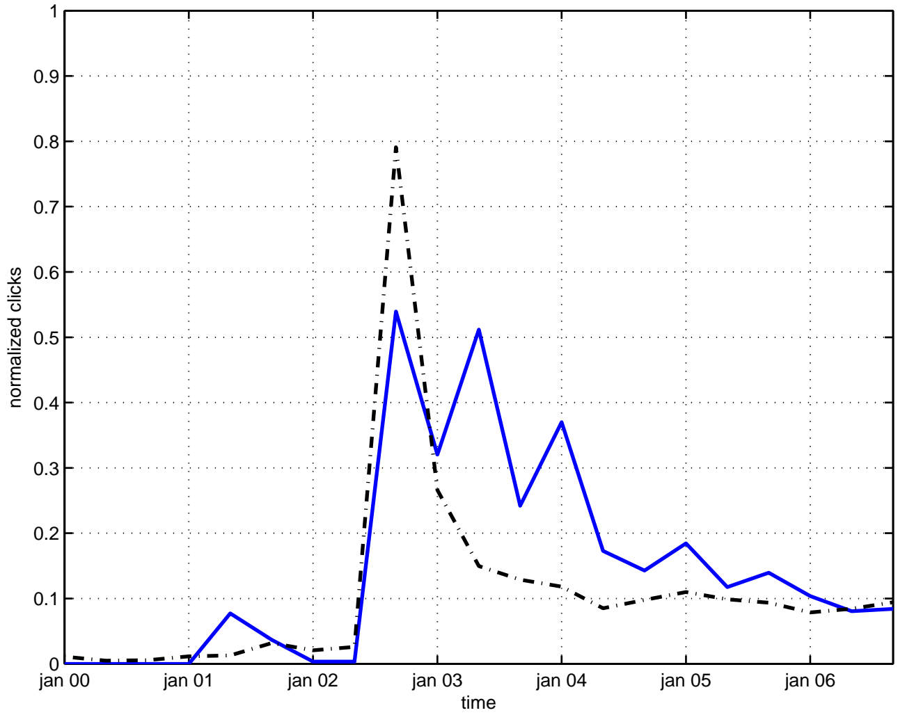
sphere symmetry
