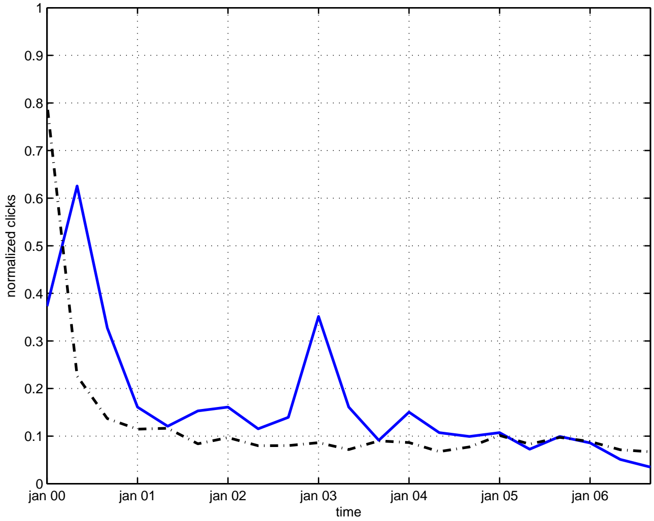
sphere spontaneous compactification
