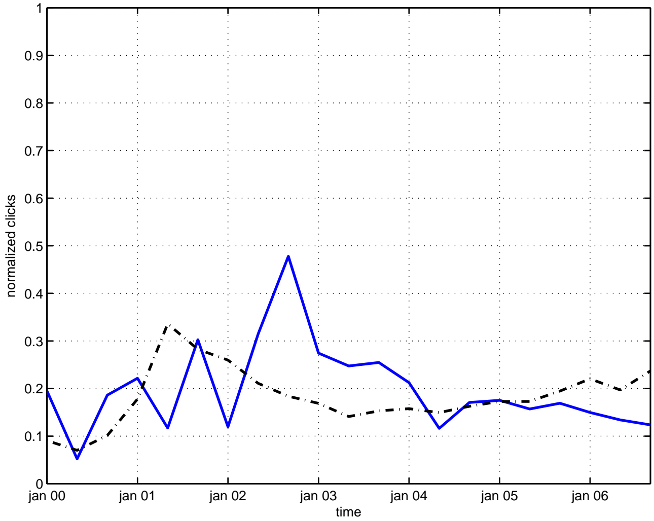
sphere space-time
