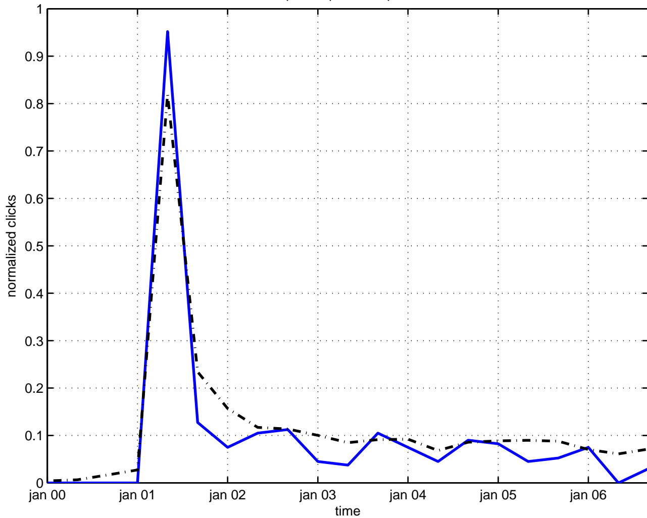
sphere quantum space
