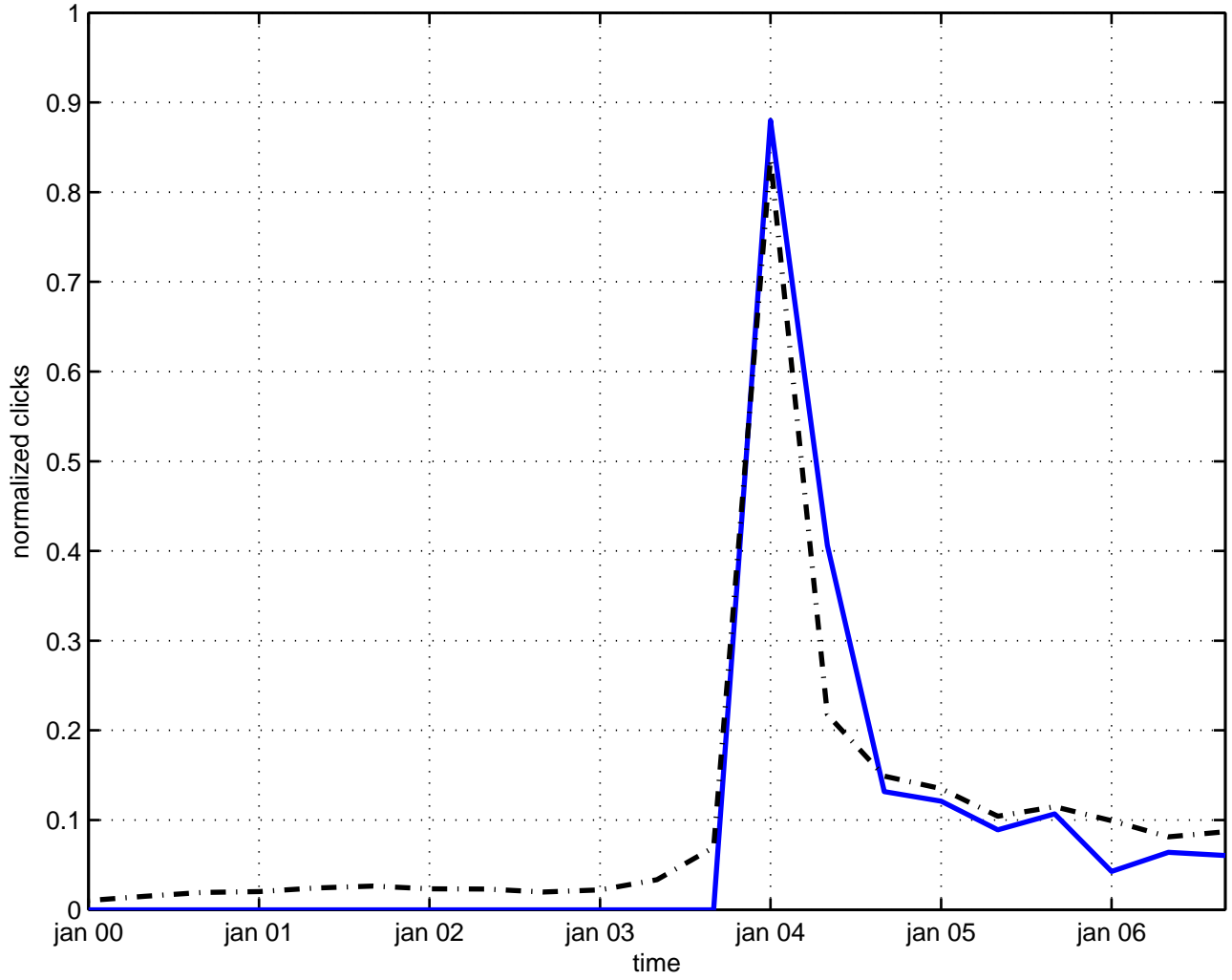
sphere fibre bundle
