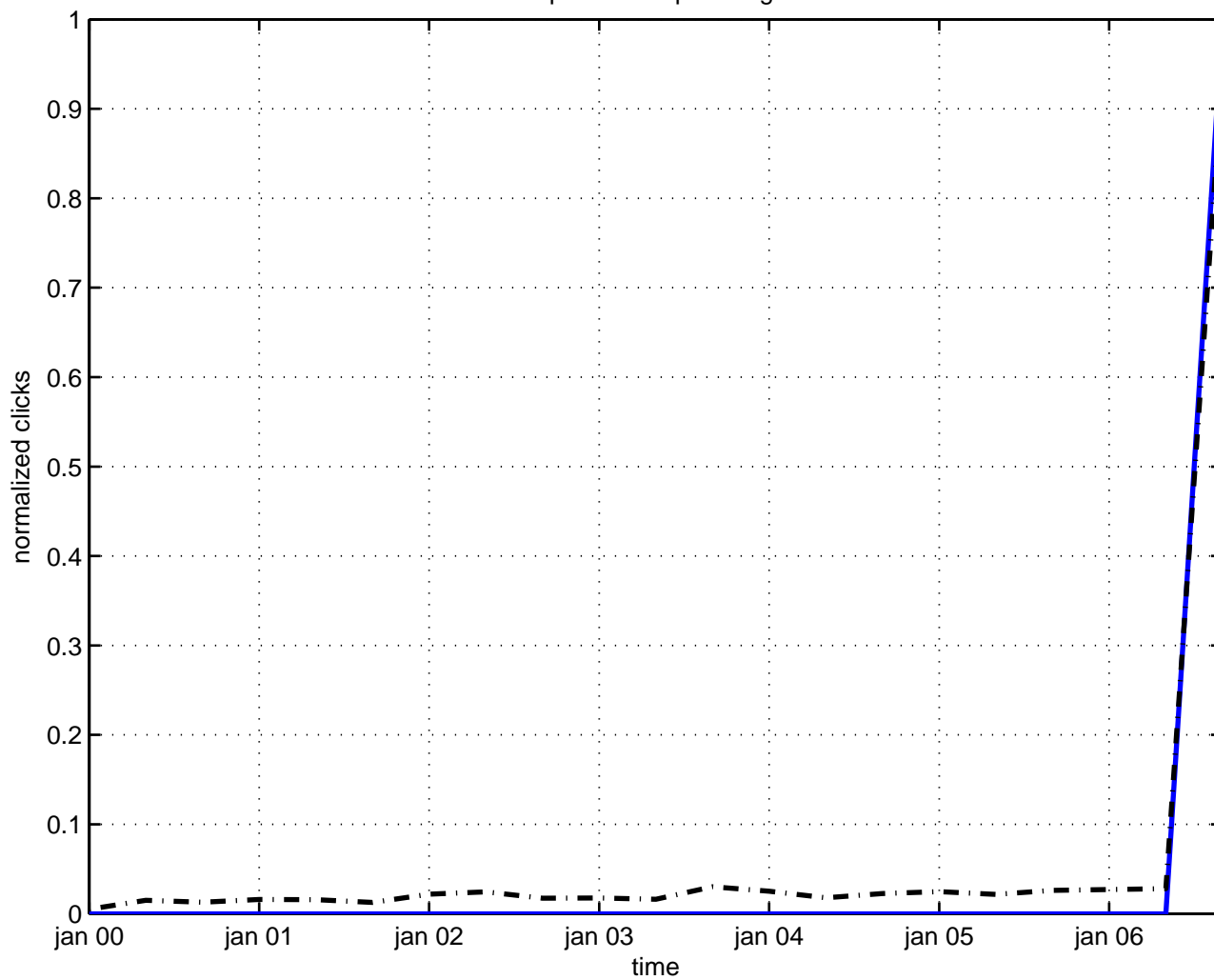
spectrum superstring
