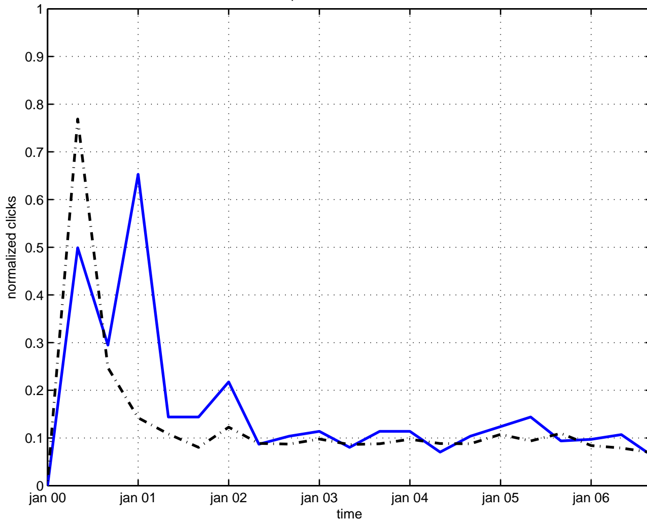
spectrum bound state
