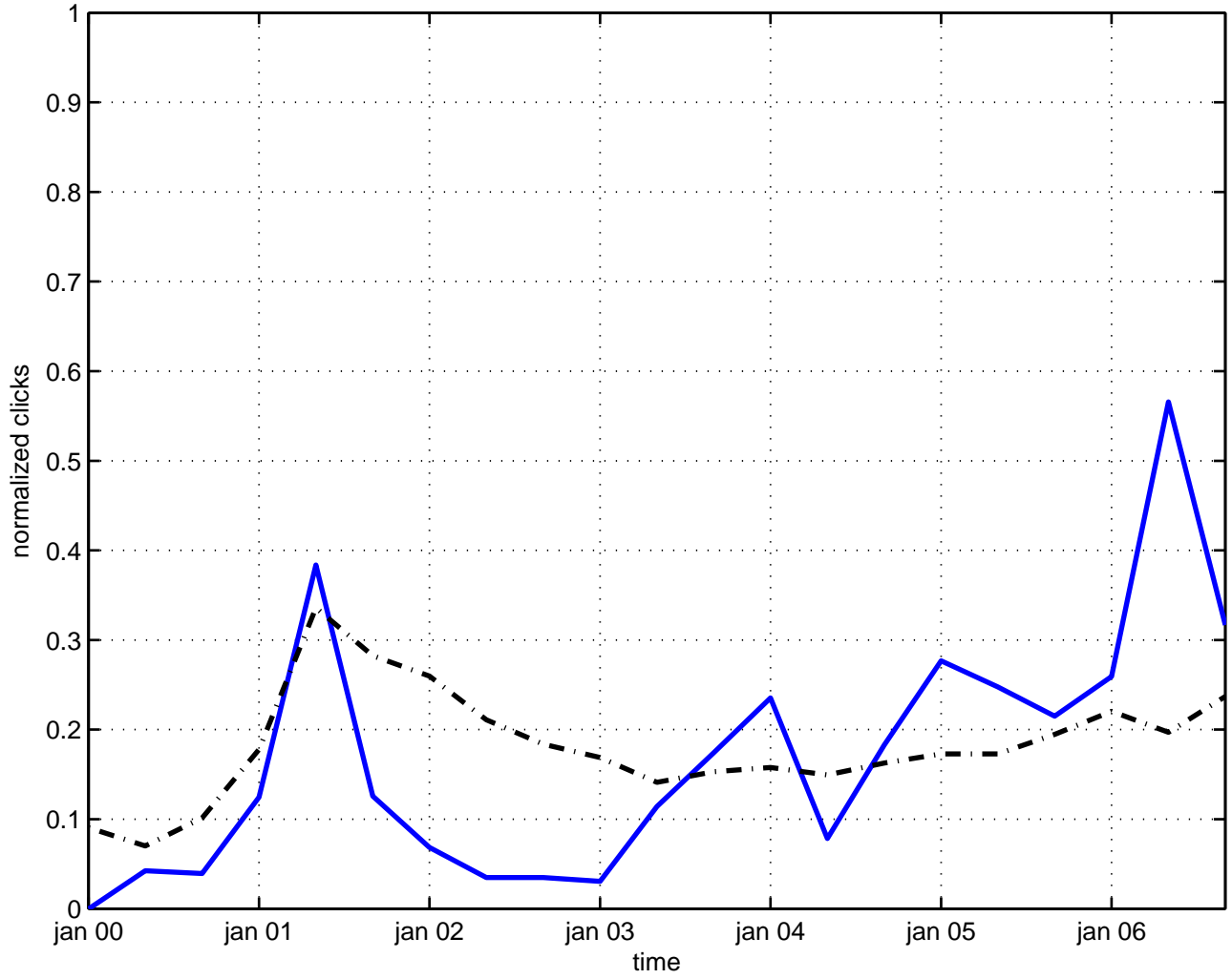
space-time symmetry
