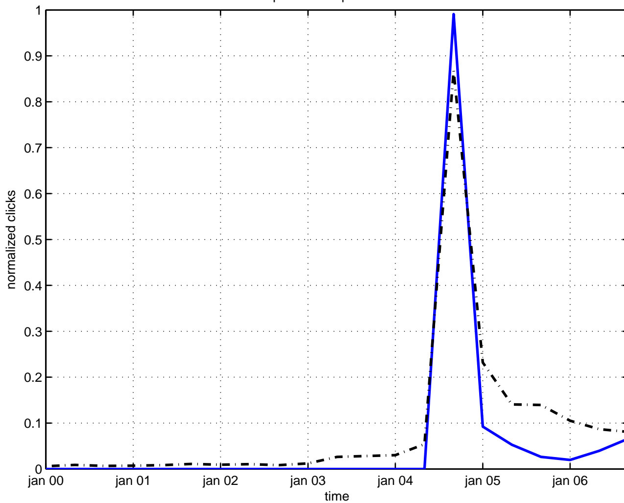
space-time quantization
