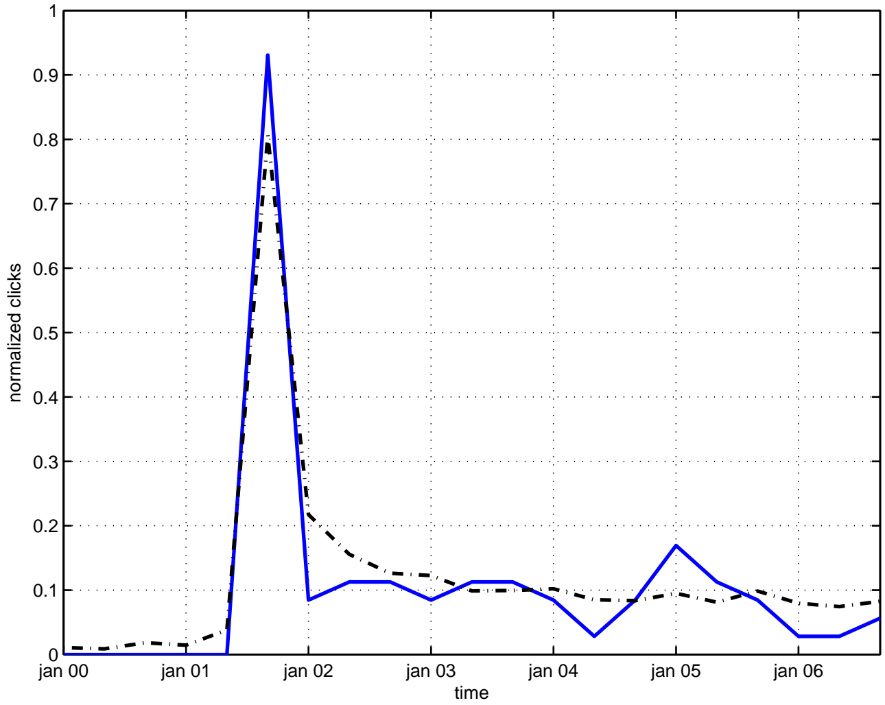
space-time monopole
