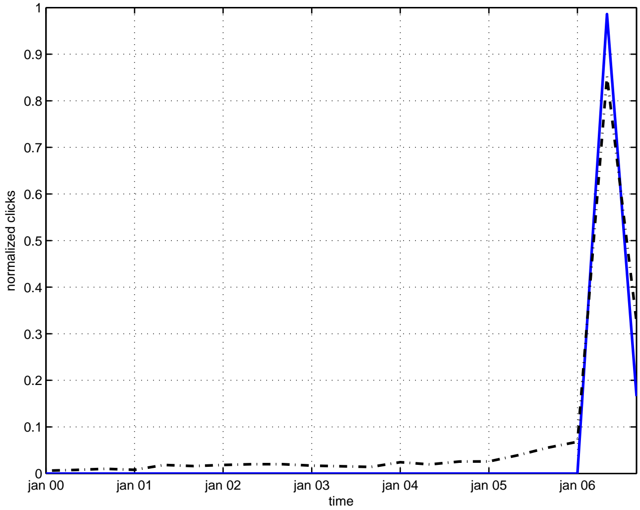
space-time group theory
