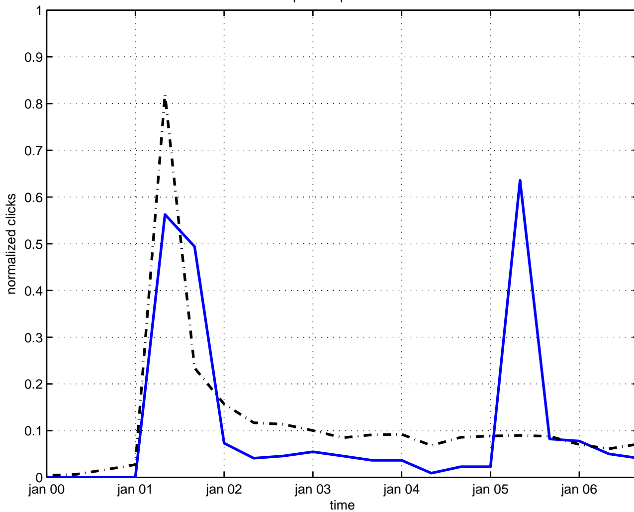
space dependence
