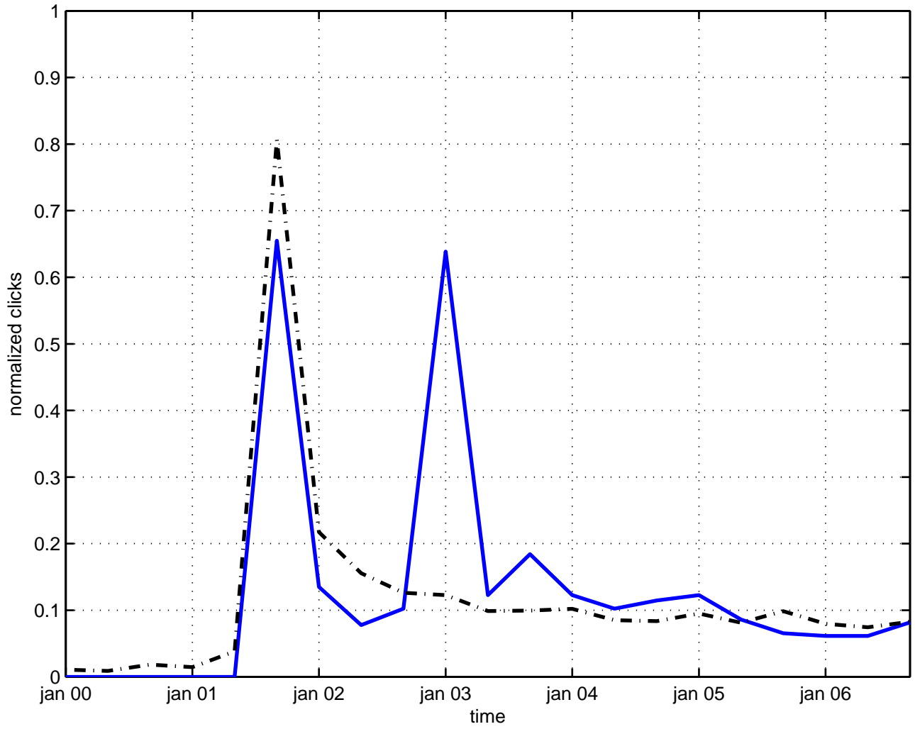
sp(n) invariance
