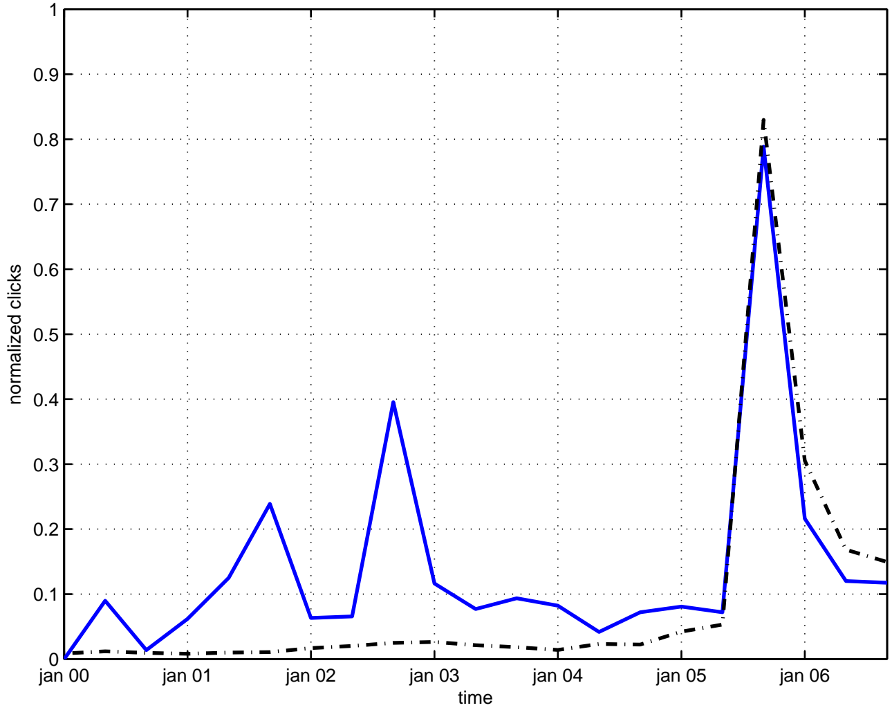
solution yang-baxter equation
