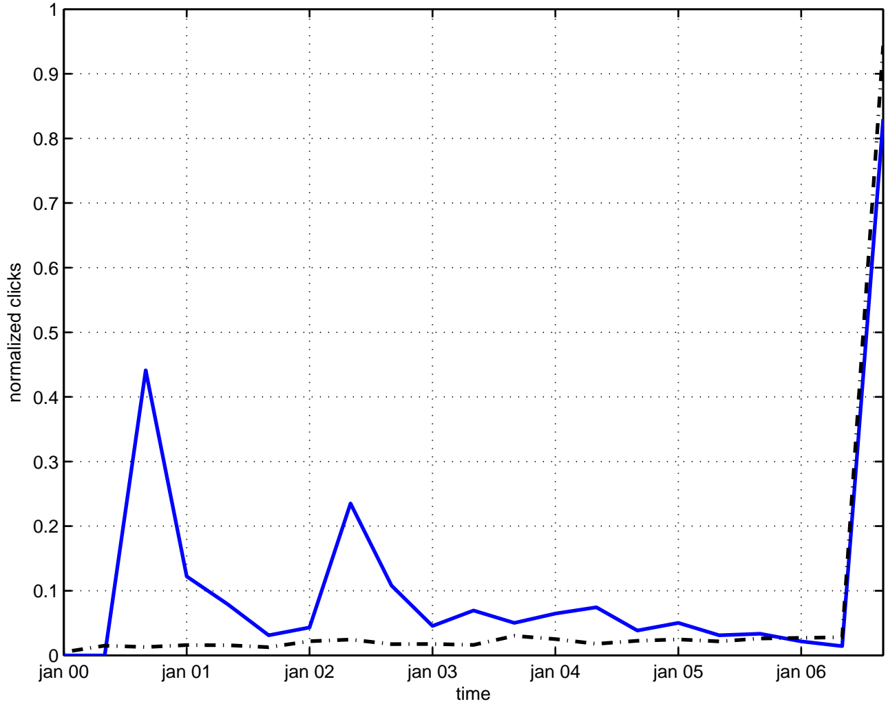
solution master equation
