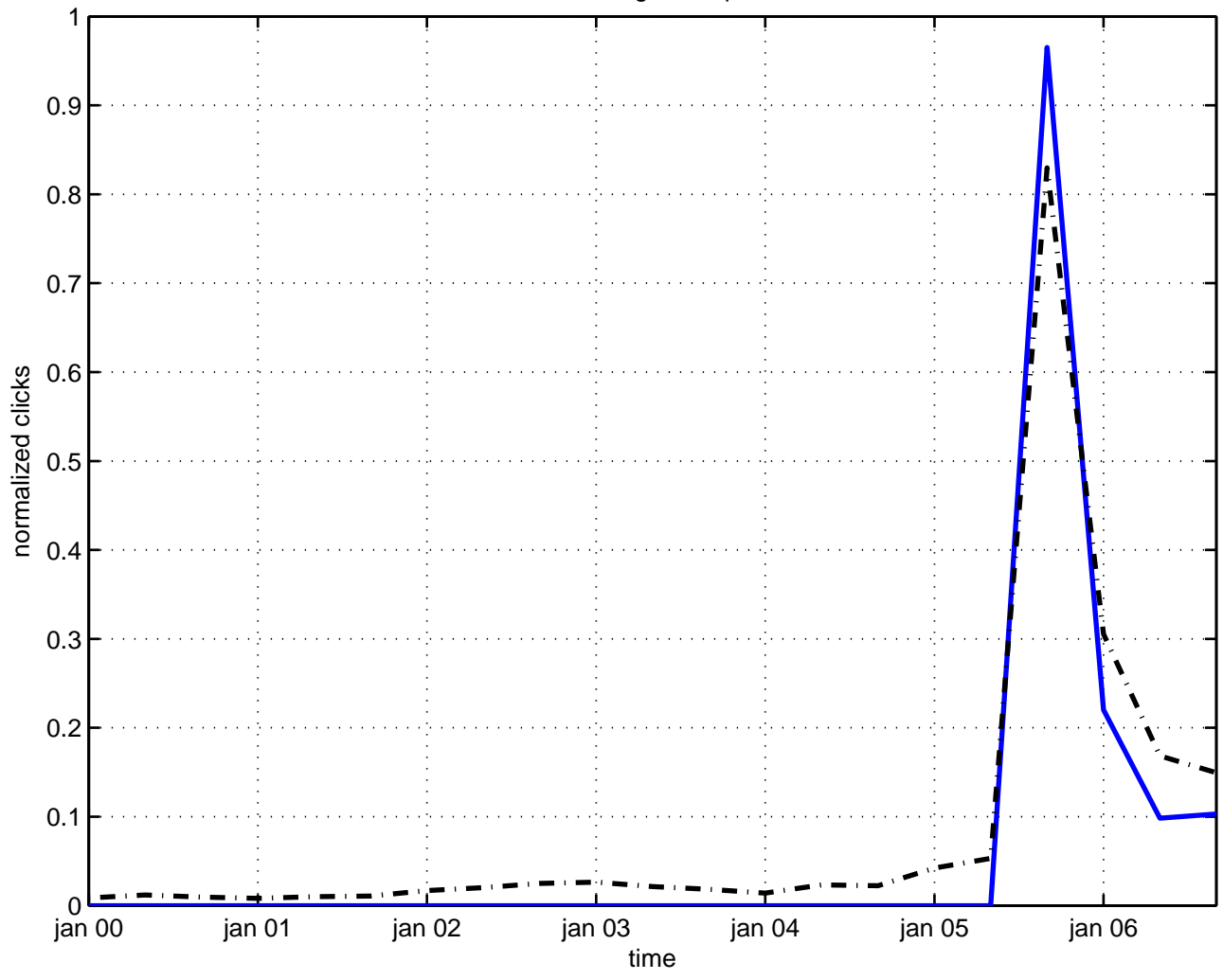
solution langevin equation
