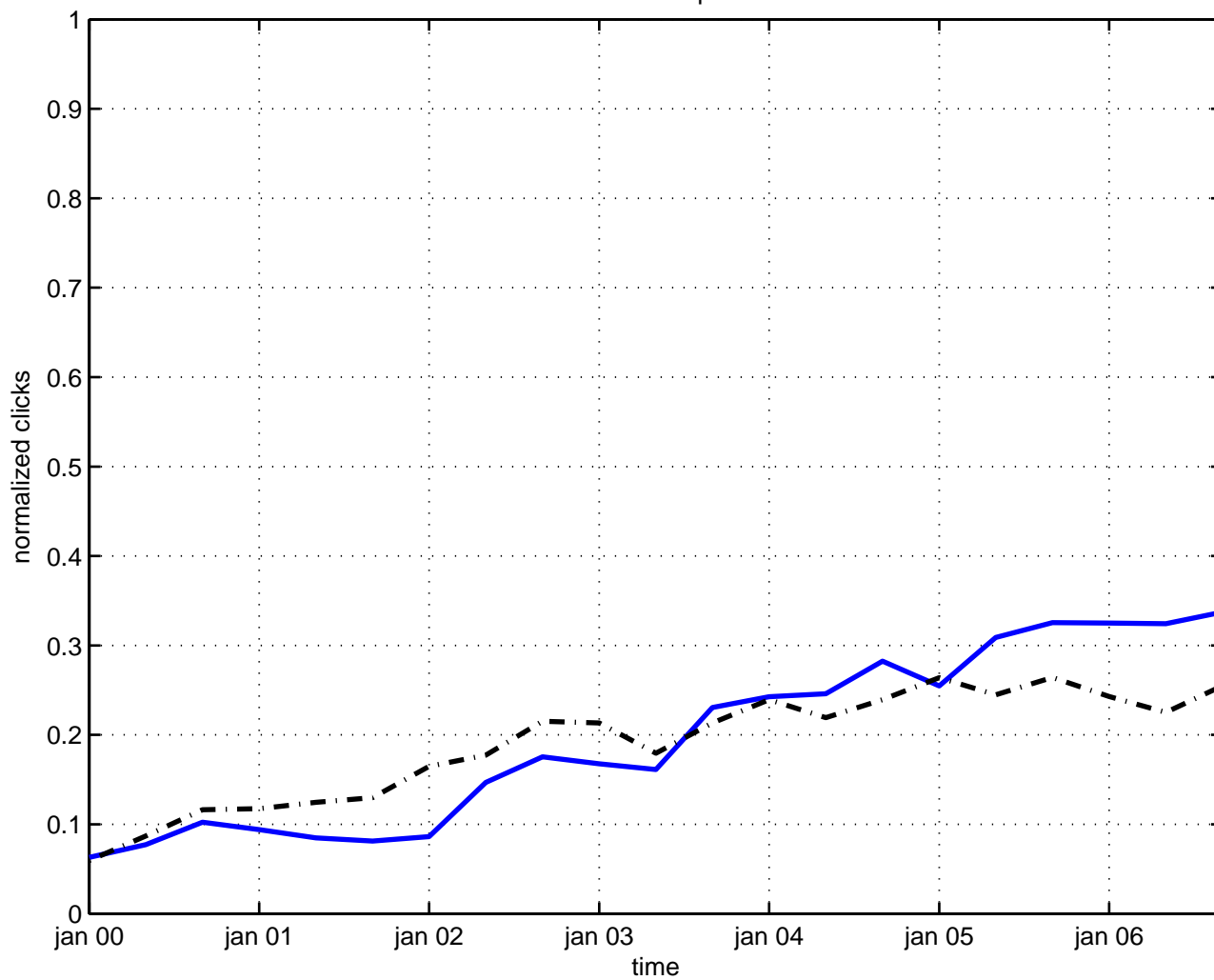
solution field equations
