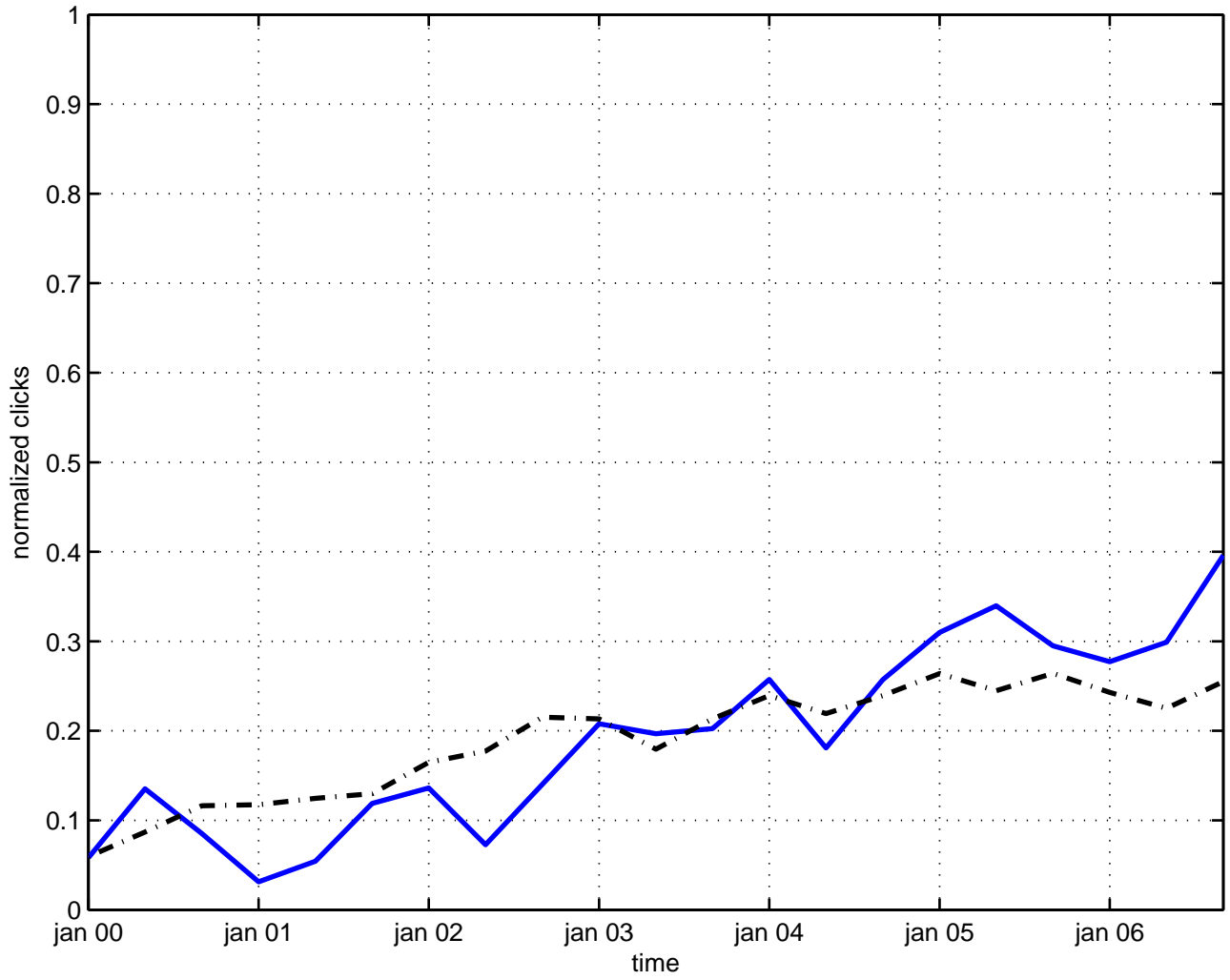
solution dirac equation
