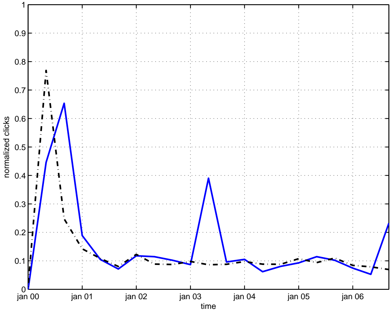
soliton schroedinger equation
