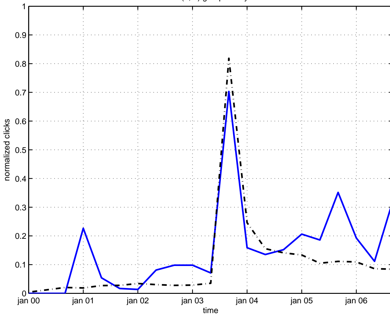
so(n,m) group theory
