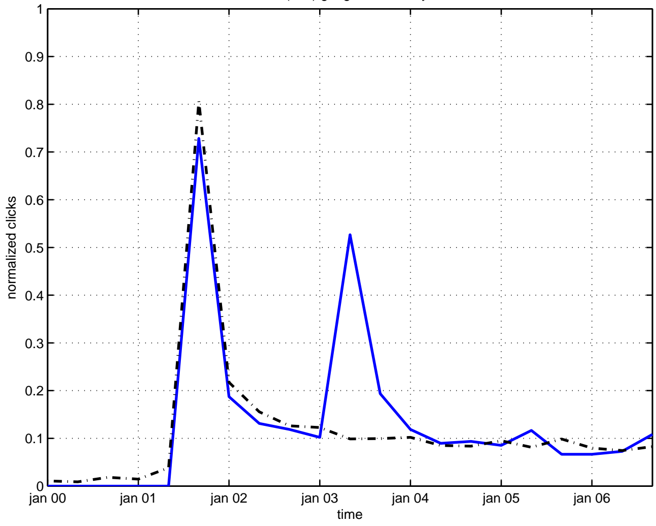
so(n,m) gauge field theory
