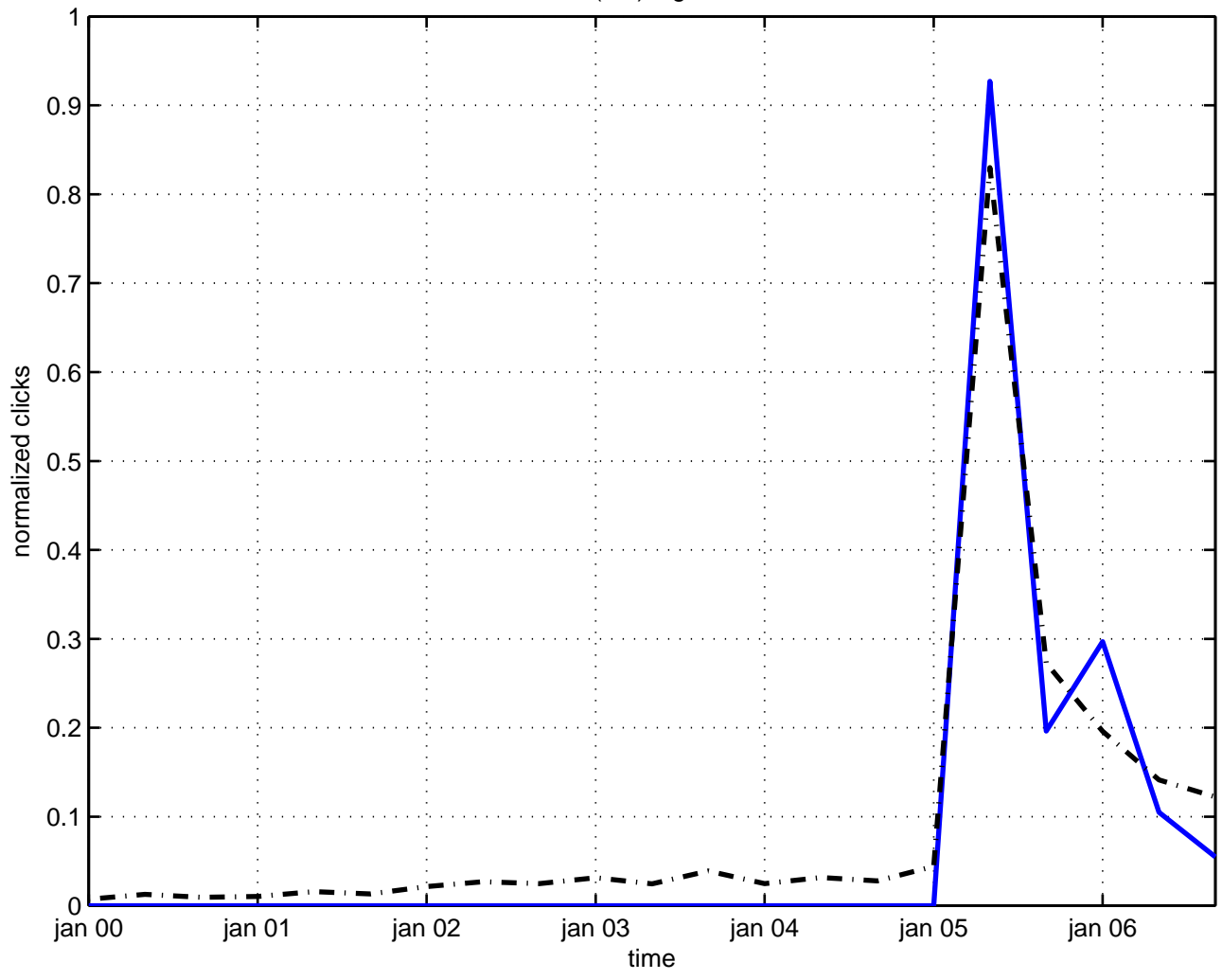
so(n,2) algebra
