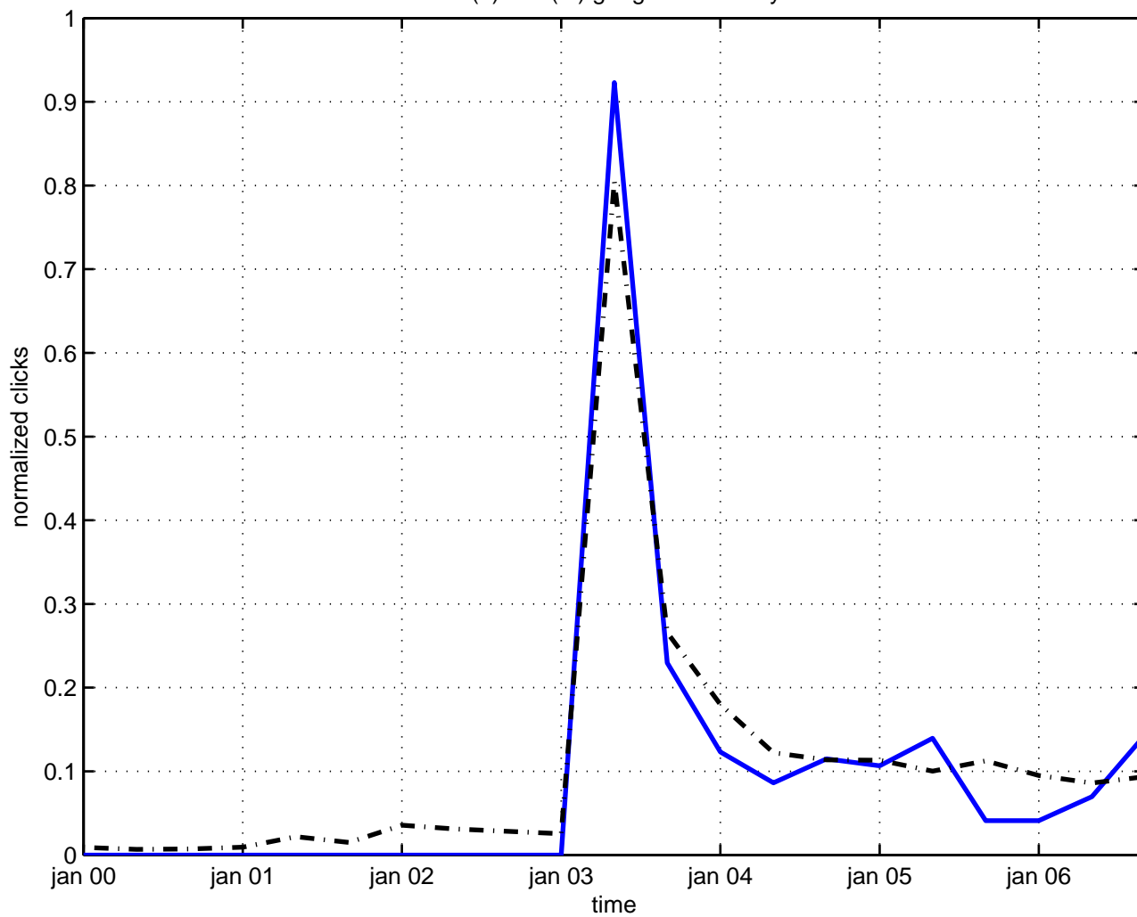
so(n) x so(m) gauge field theory
