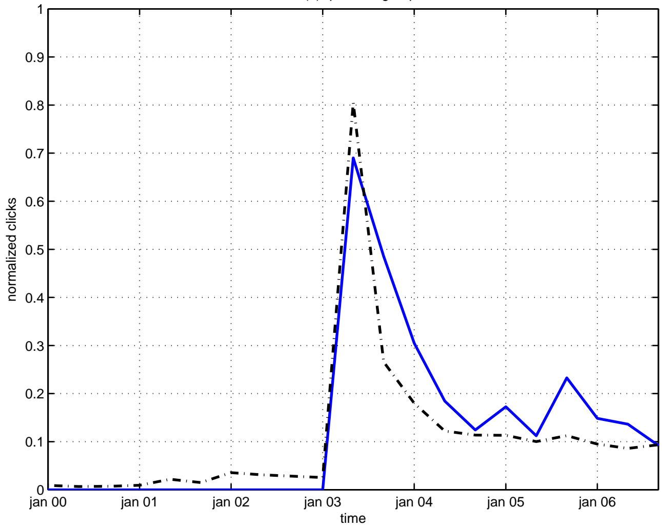
so(n) quantum group
