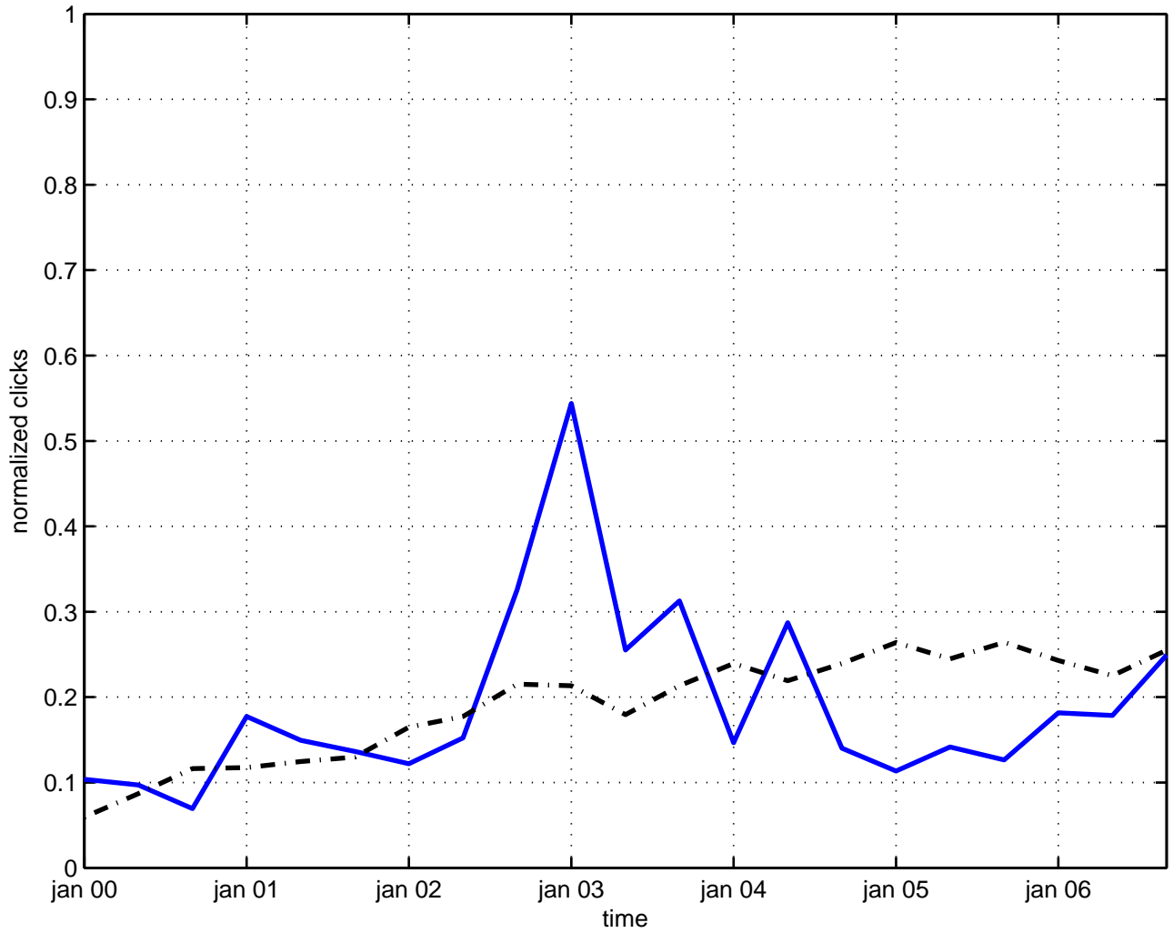
so(n) gauge field theory
