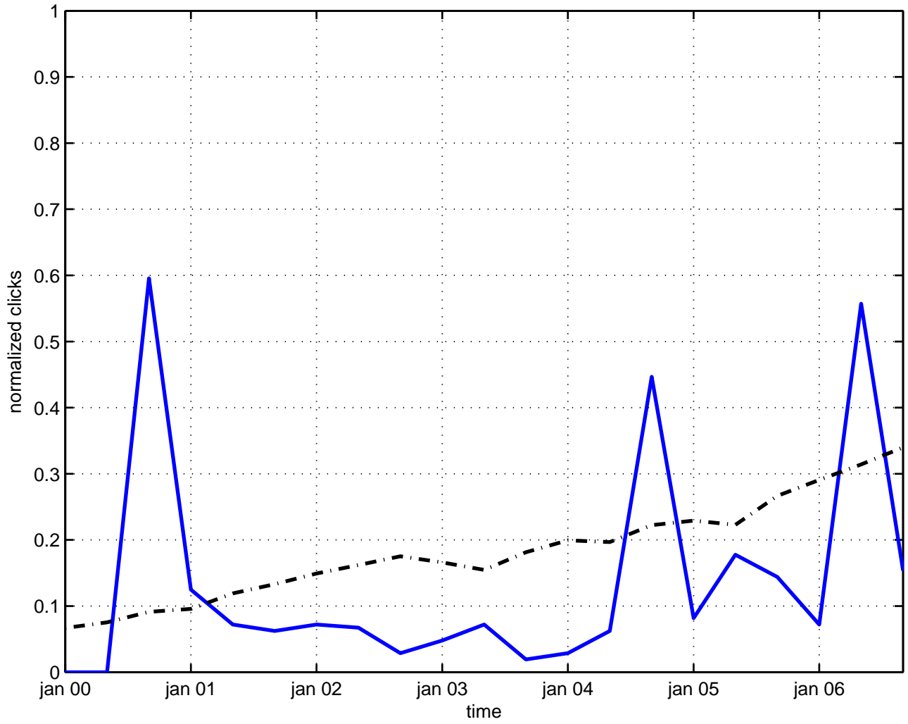
so(n) algebra
