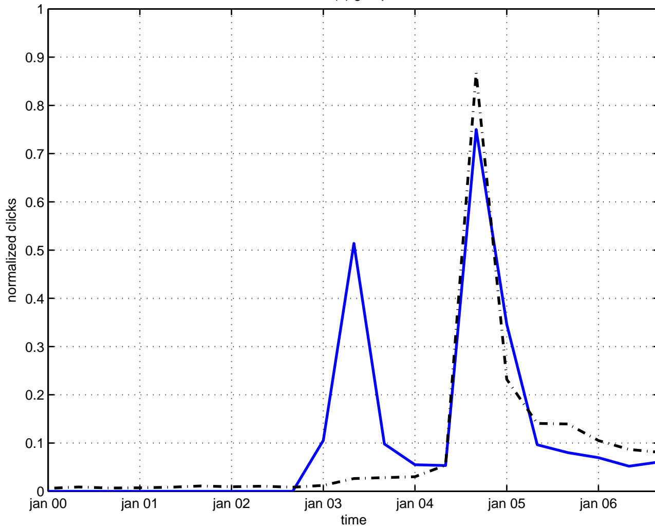
so(9) group
