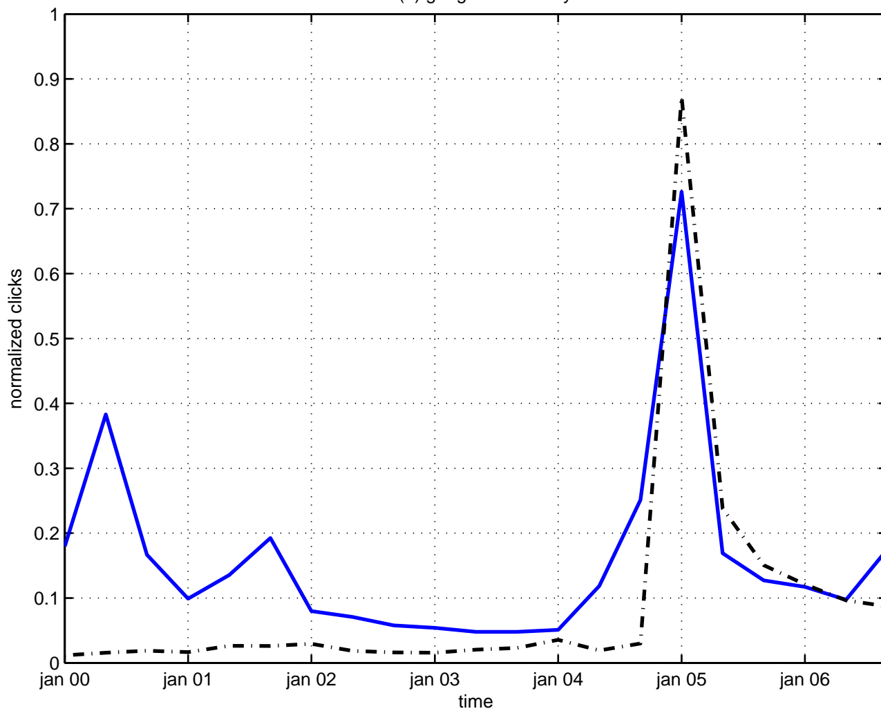
so(5) gauge field theory
