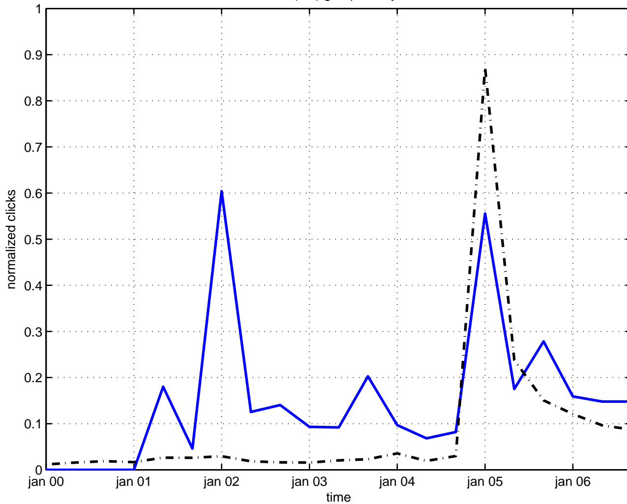
so(4,2) group theory
