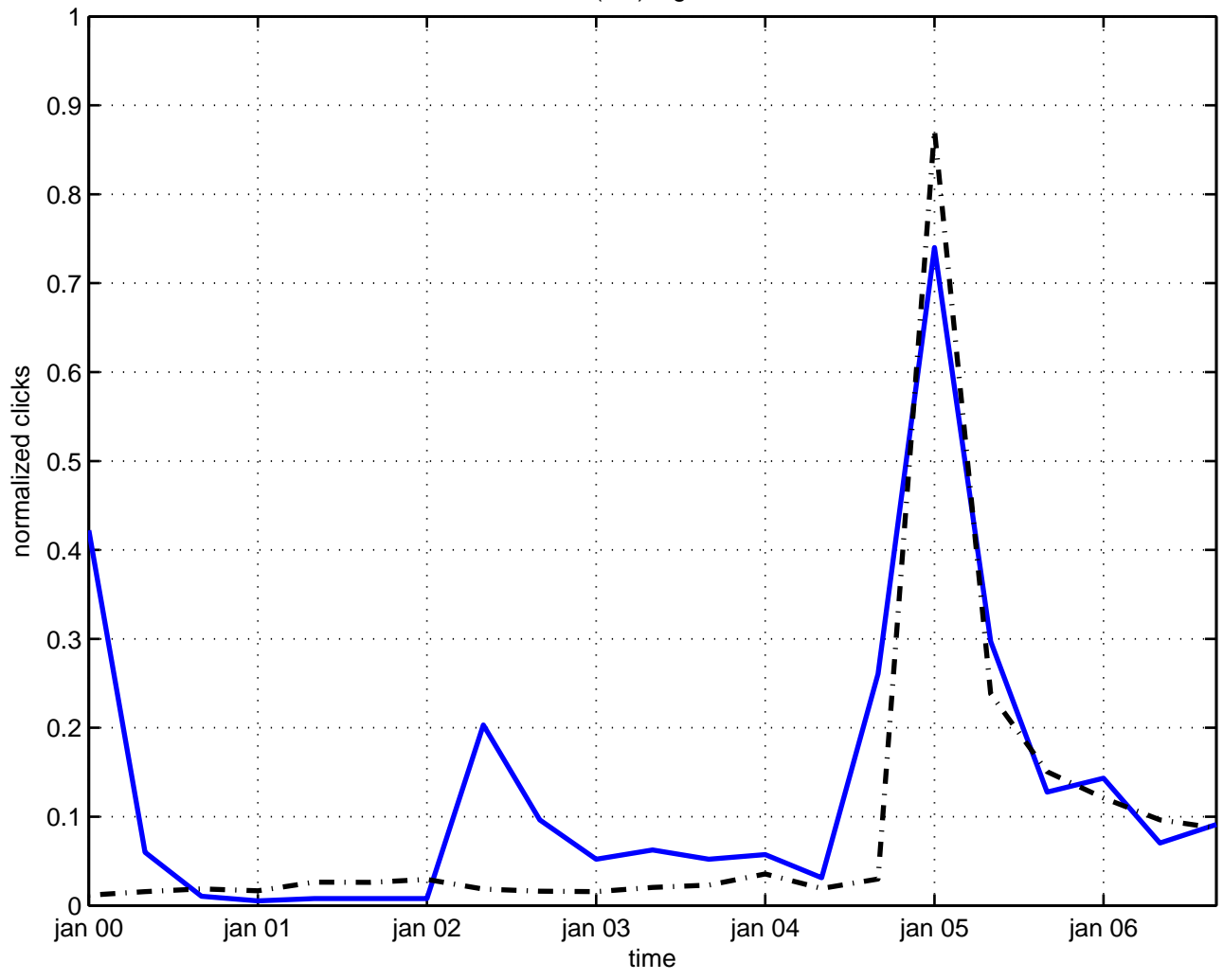
so(4,2) algebra
