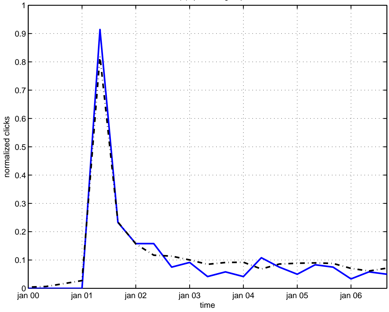
so(4) quantum group
