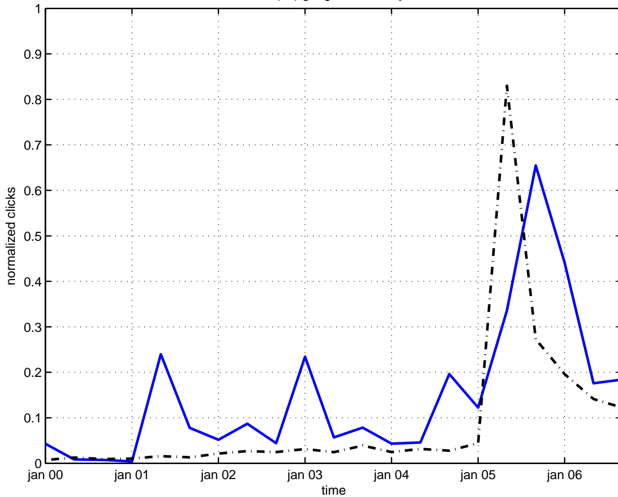
so(32) gauge field theory
