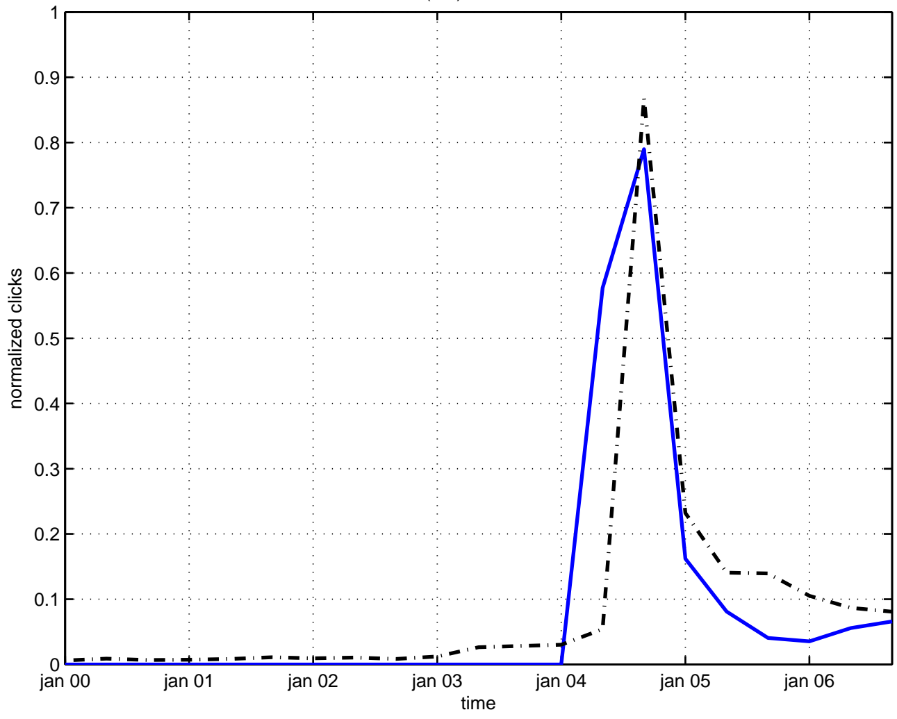
so(3,2) invariance
