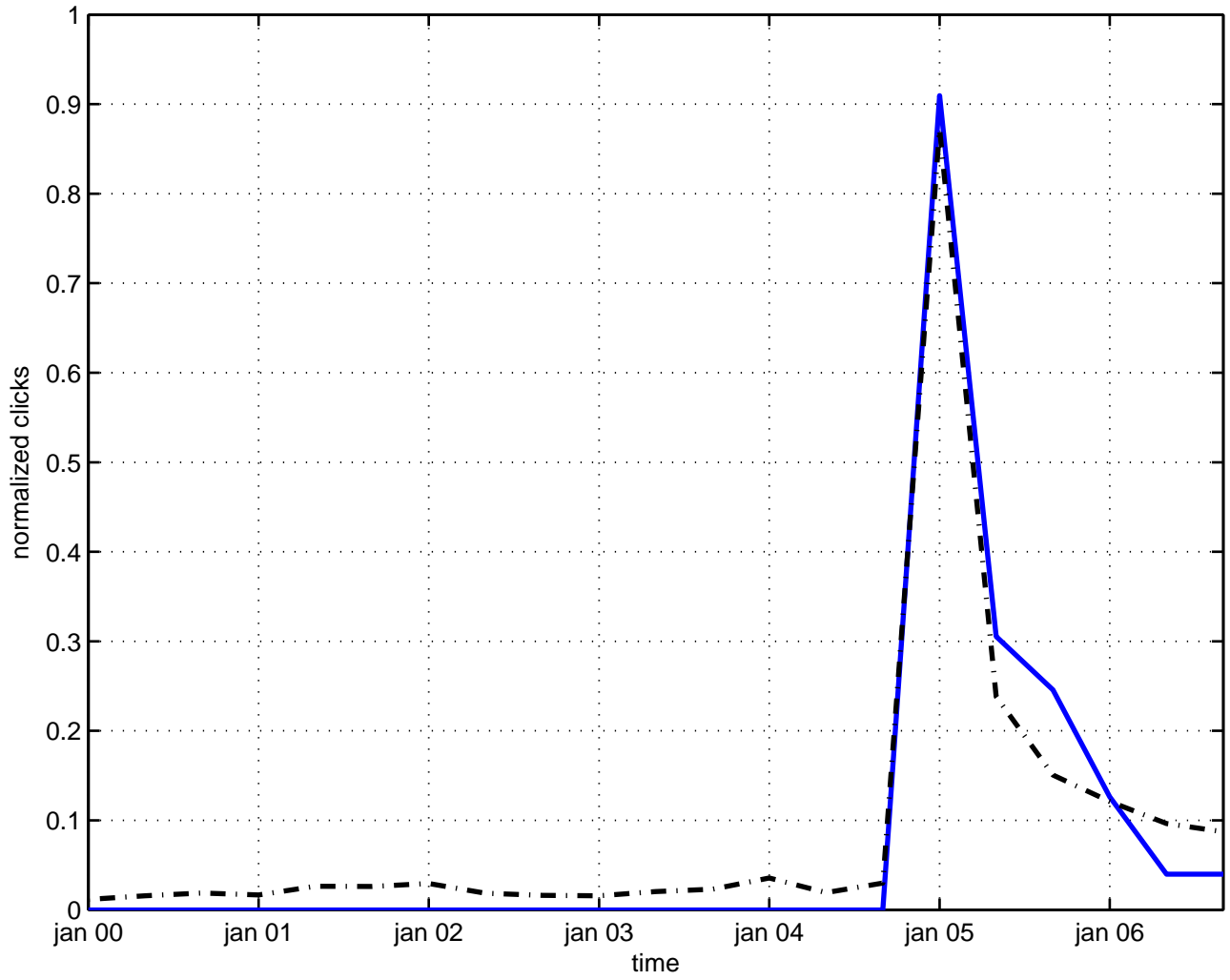
so(3) x so(3) symmetry
