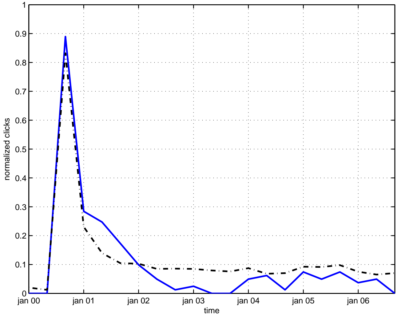
so(3) x so(3) gauge field theory
