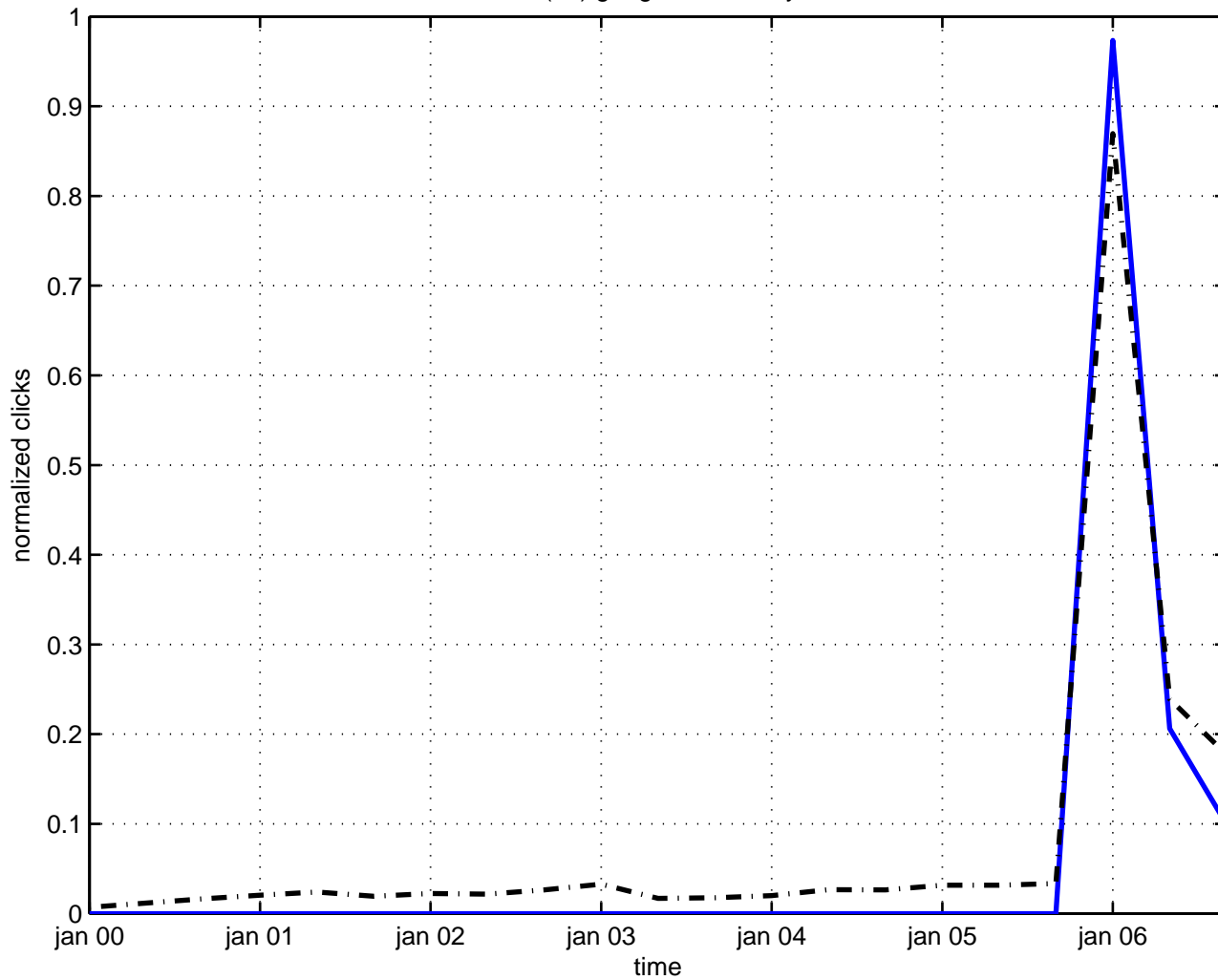
so(24) gauge field theory
