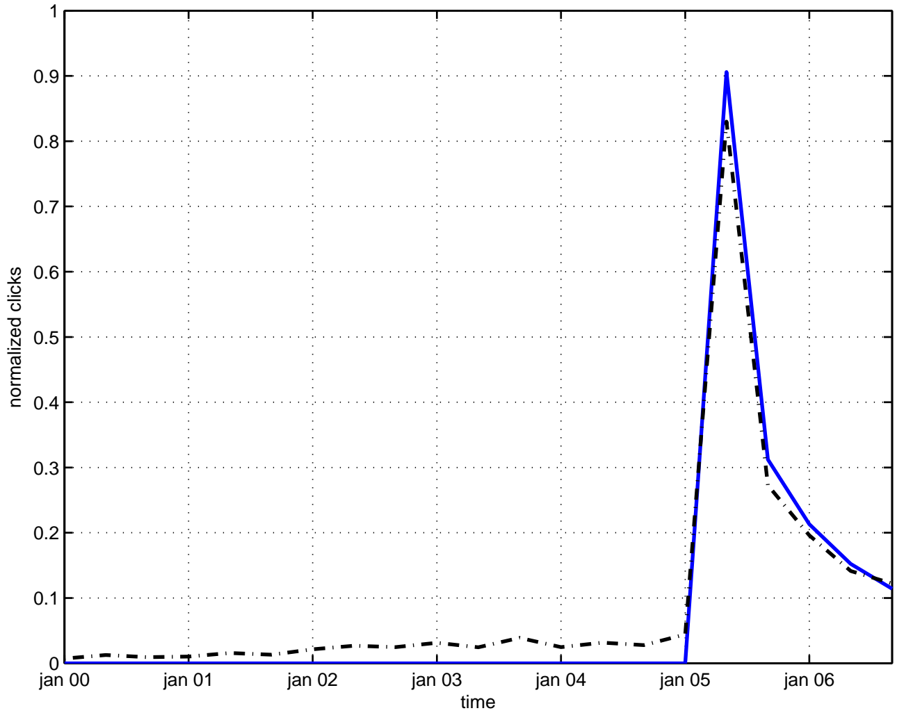
so(2,n) group theory
