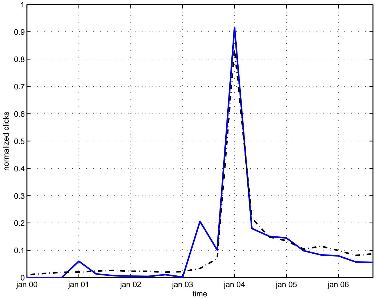
so(2,2) symmetry
