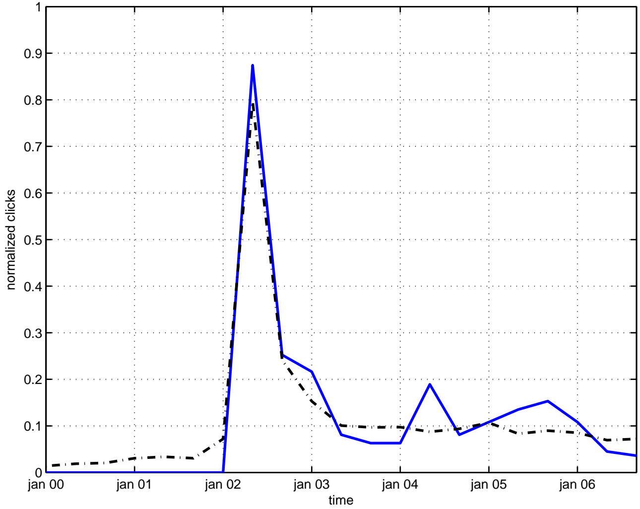
so(14) grand unified theory
