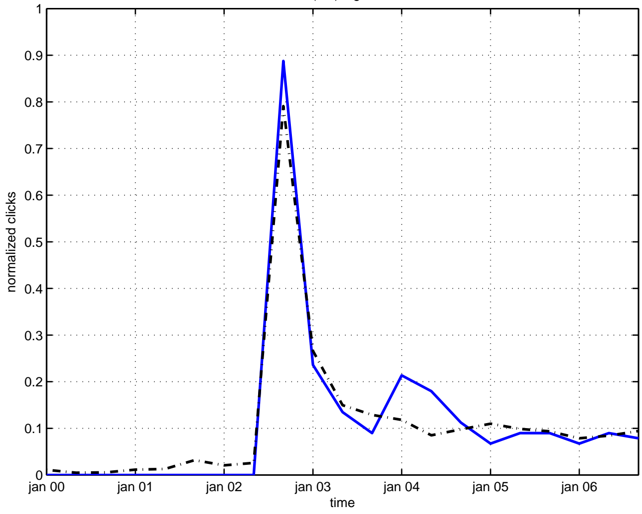
so(1,4) algebra
