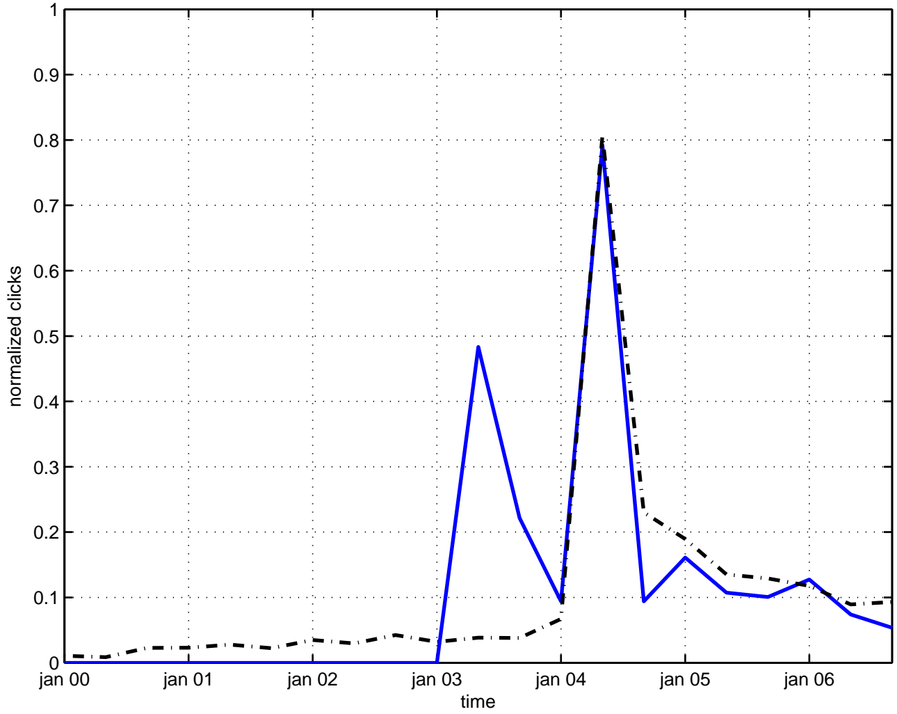
so(1,2) symmetry
