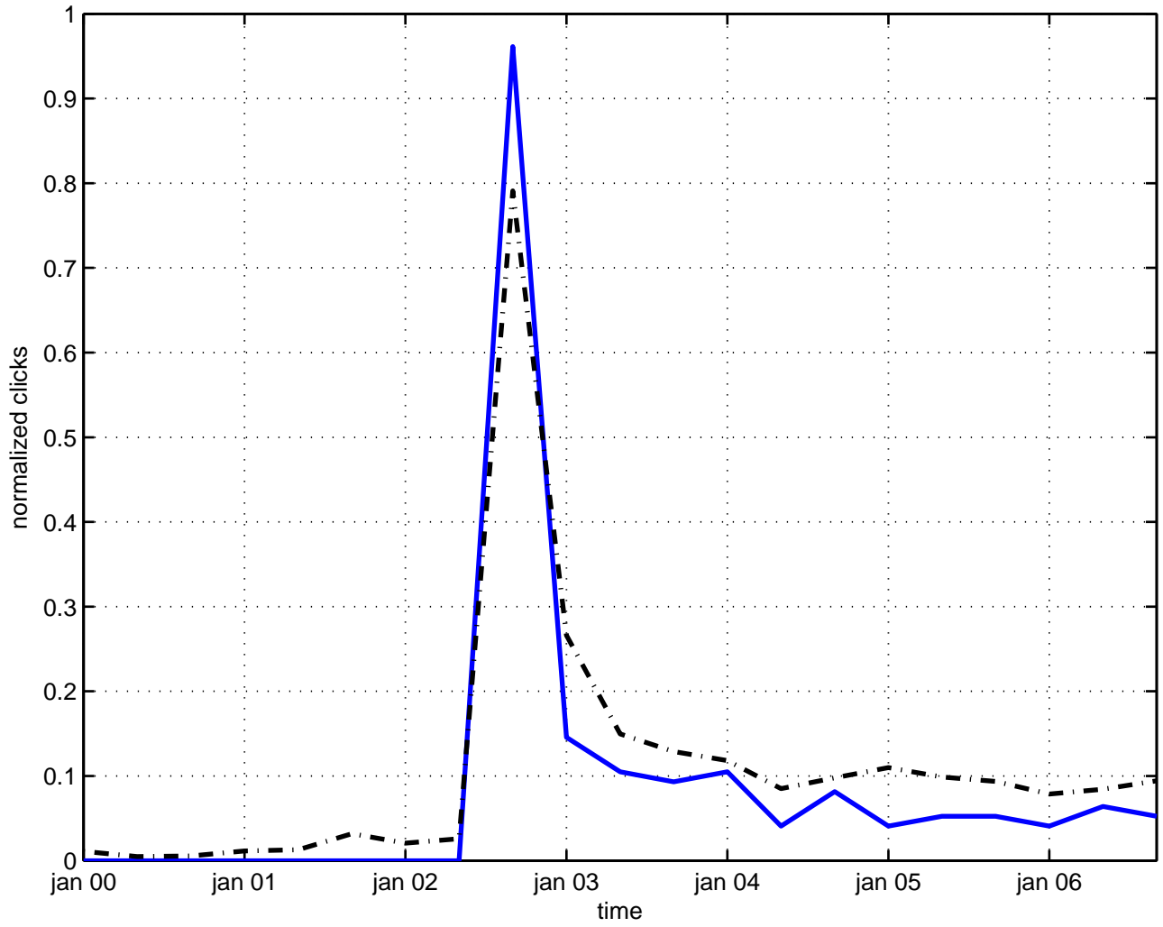
so(1,2) group theory
