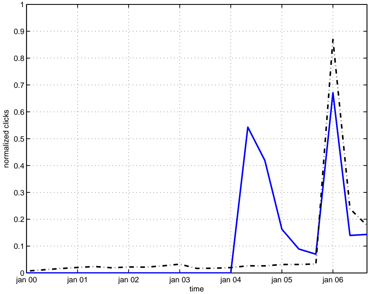
snyder space-time
