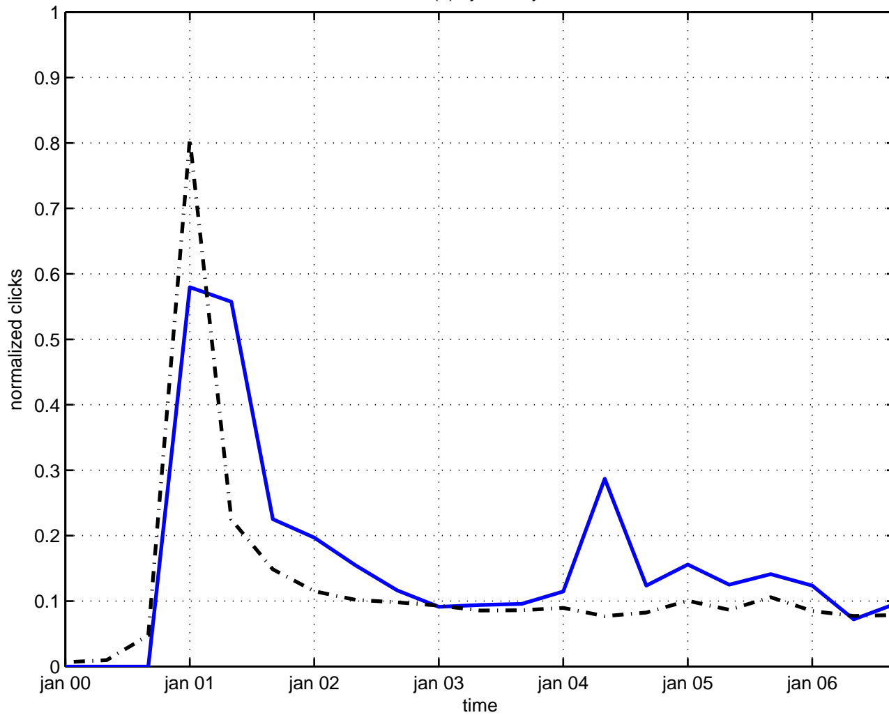
sl(3) symmetry
