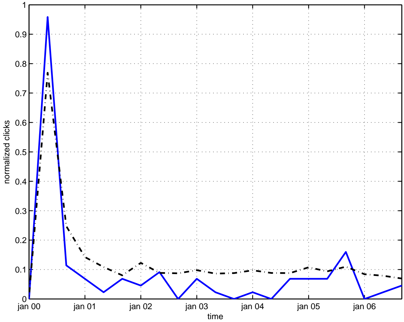
sl(3) quantum group
