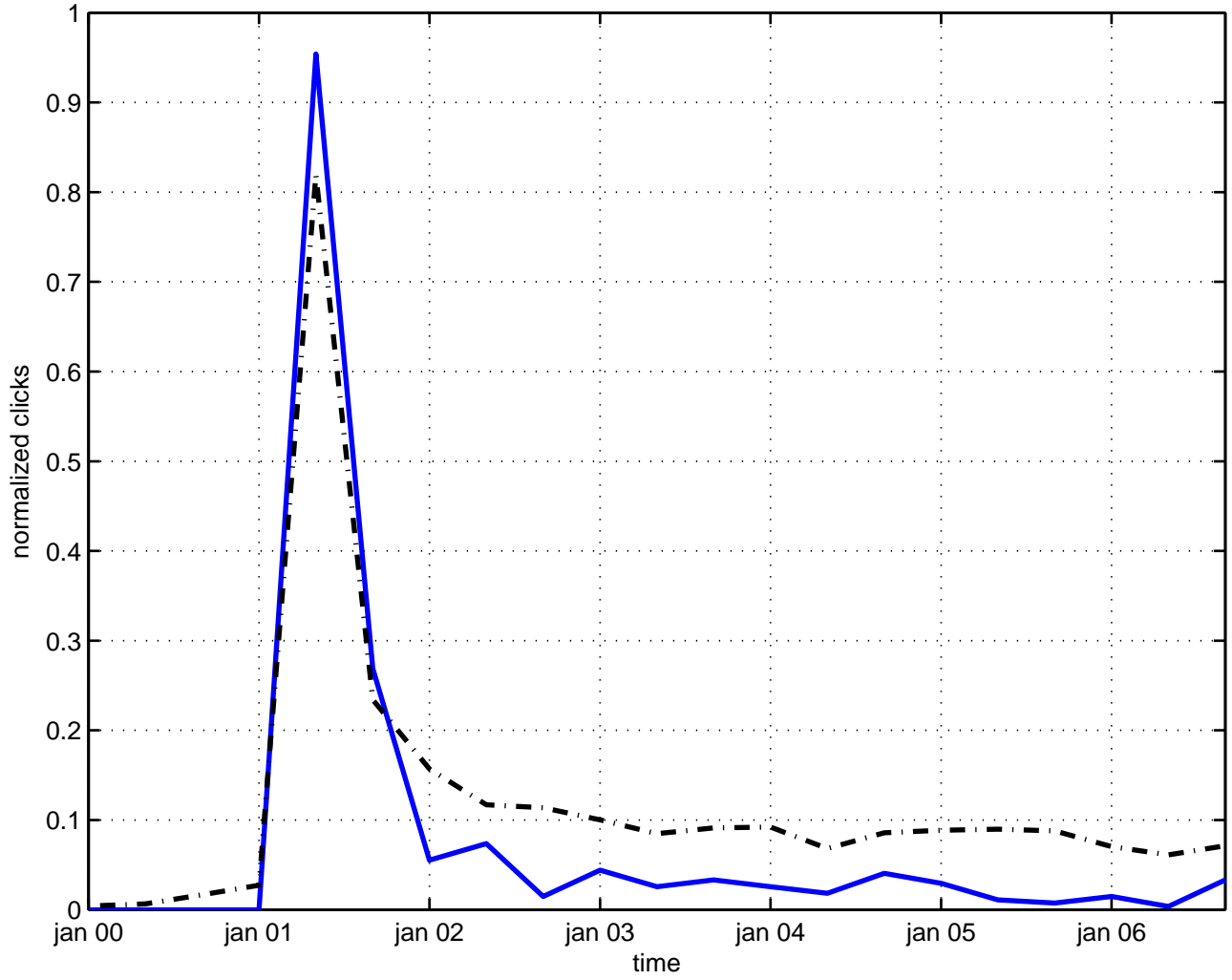
sl(2,z) s-duality
