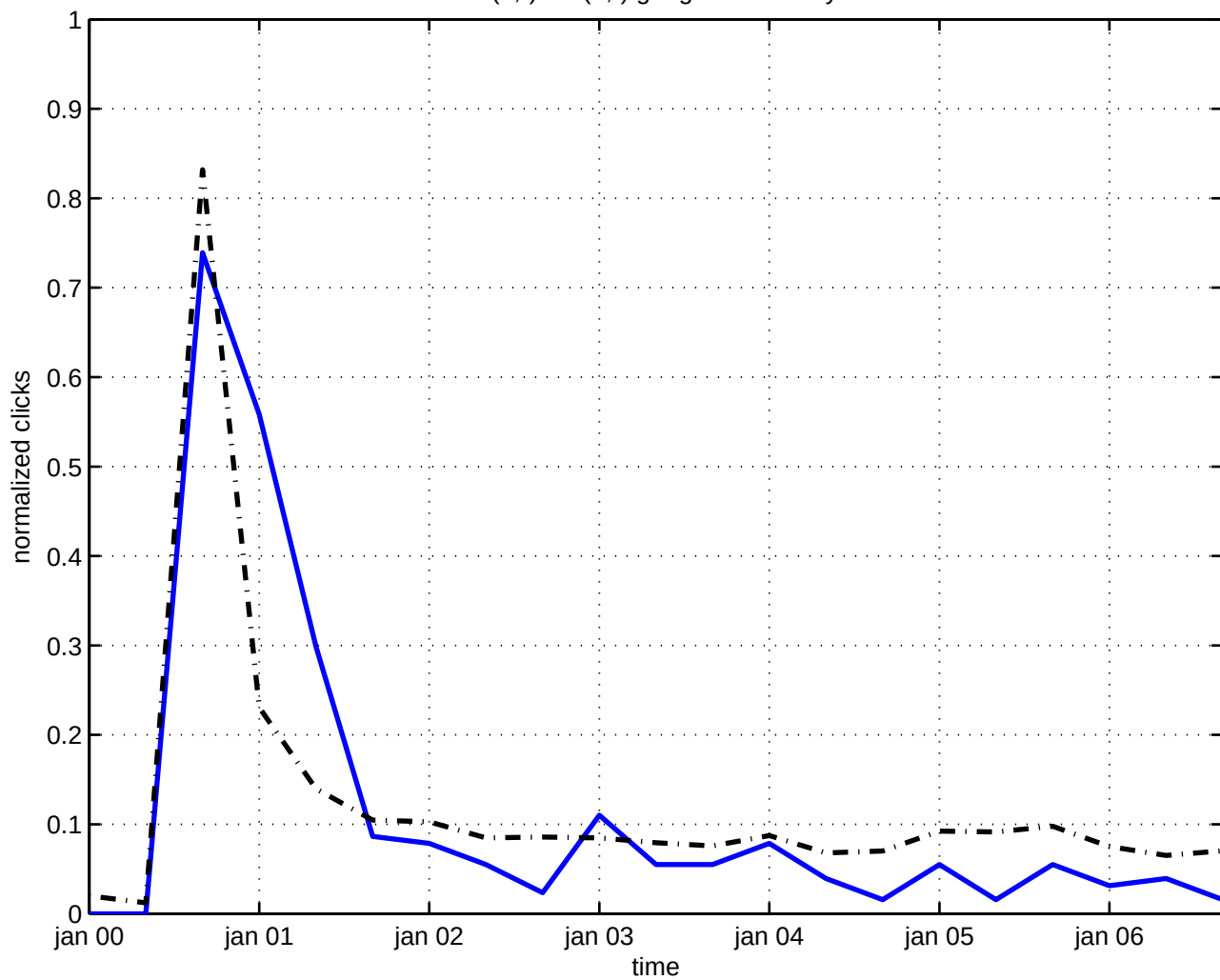
sl(2,r) \times sl(2,r) gauge field theory
