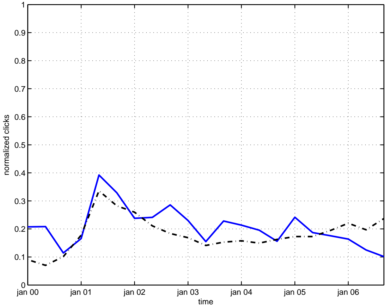
sl(2,r) wess-zumino-witten model
